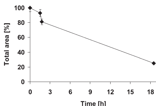
Figure 3. Decomposition of \alpha -ketoadipyl-7-ACA in the reaction conditions. 4 mL of \alpha -ketoadipyl-7-ACA were incubated at pH 7 and 25 °C. The reduction of the peak area corresponding to \alpha -ketoadipyl-7-ACA was monitored by HPLC as described in the Experimental Section.
