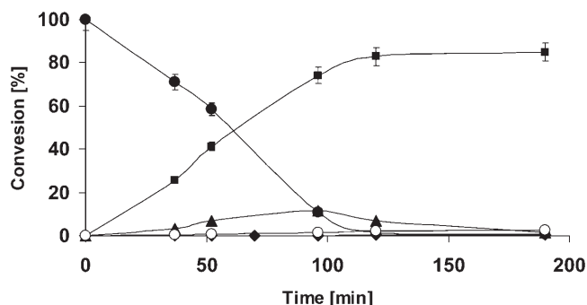
Figure 4. Reaction course of the conversion of cephalosporin C into 7-aminocephalosporanic acid using the trienzymatic, one-pot process. The reaction was carried out as described in the Experimental Section; ■: 7-ACA. ●: CPC. ▲: \alpha -ketoadipyl-7-ACA; ○: side products and ◆: GL-7-ACA.
