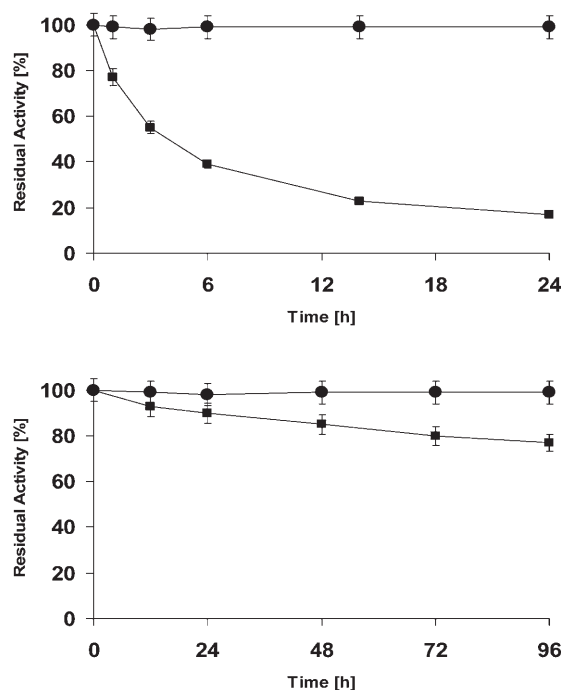
Figure 1. Inactivation of DAAO ( top ) and GAC ( bottom ) by hydrogen peroxide. 4 IU DAAO immobilized on glyoxyl agarose and 12 IU/mL PEI-GAC-glut derivative were separately incubated with and without 10 mM hydrogen peroxide at pH 7 and 25 °C. ●: enzyme without hydrogen peroxide and ■: enzyme with hydrogen peroxide.
