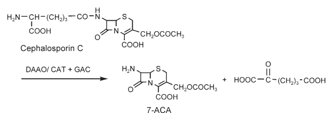
Scheme 1. Different routes for the conversion of CPC to 7-ACA.
