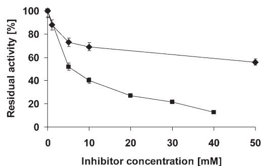
Figure 2. Effect of glutaric acid on the \alpha -ketoadipyl-7-ACA amidase and GL-7-ACA amidase activities. ◆: GL-7-ACA amidase activity and ■: \alpha -ketoadipyl-7-ACA amidase activity. Further details are described in the Experimental Section.
